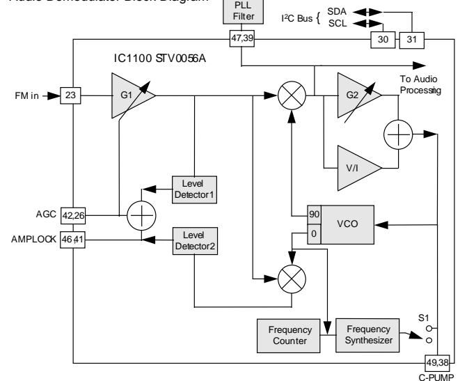
Audio Demodulator Block Diagram
